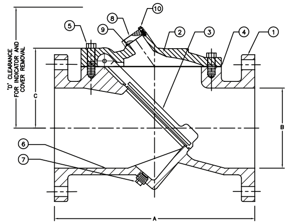
SECTION F-F
